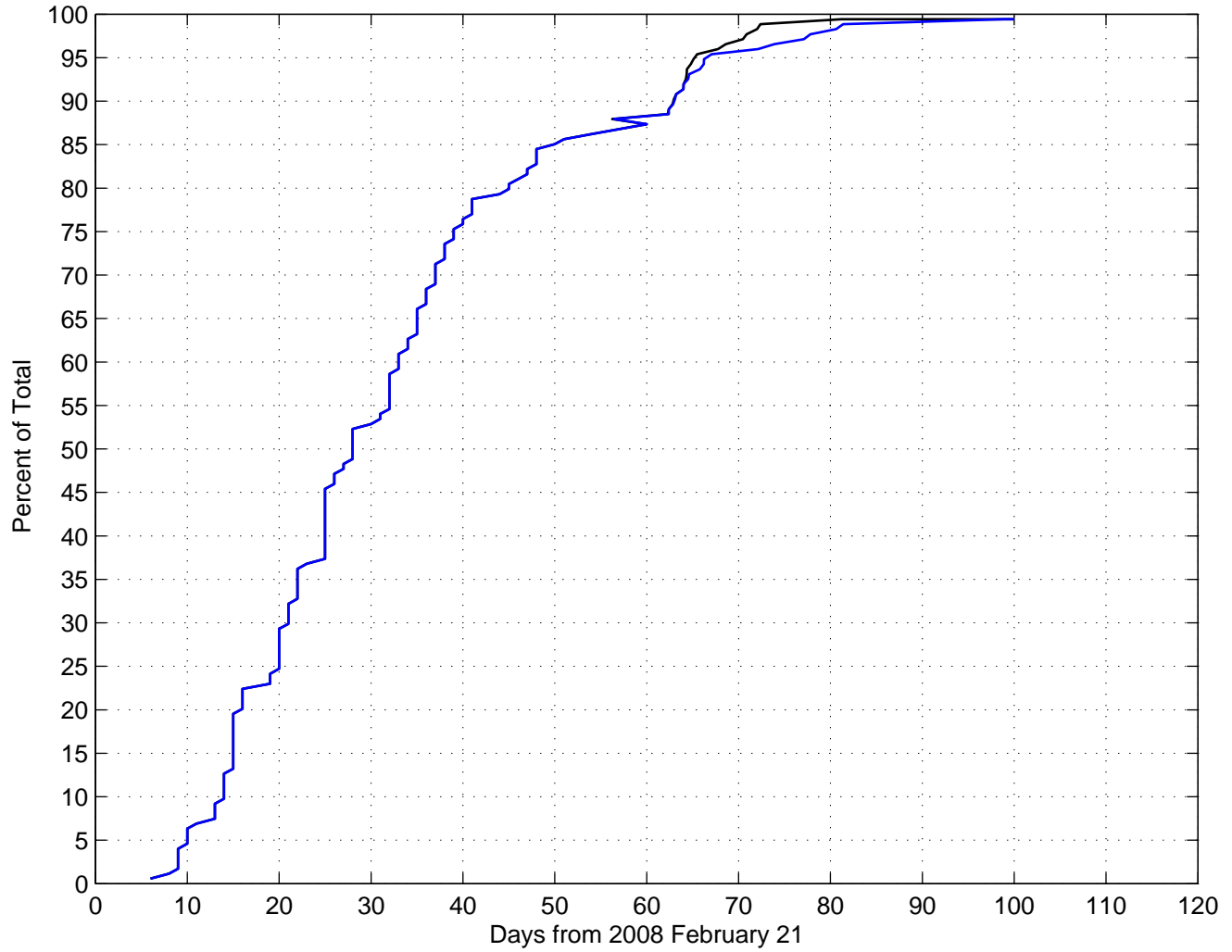
Lifetime Plot of USA 193 (2006–057) Debris (174 pieces)
