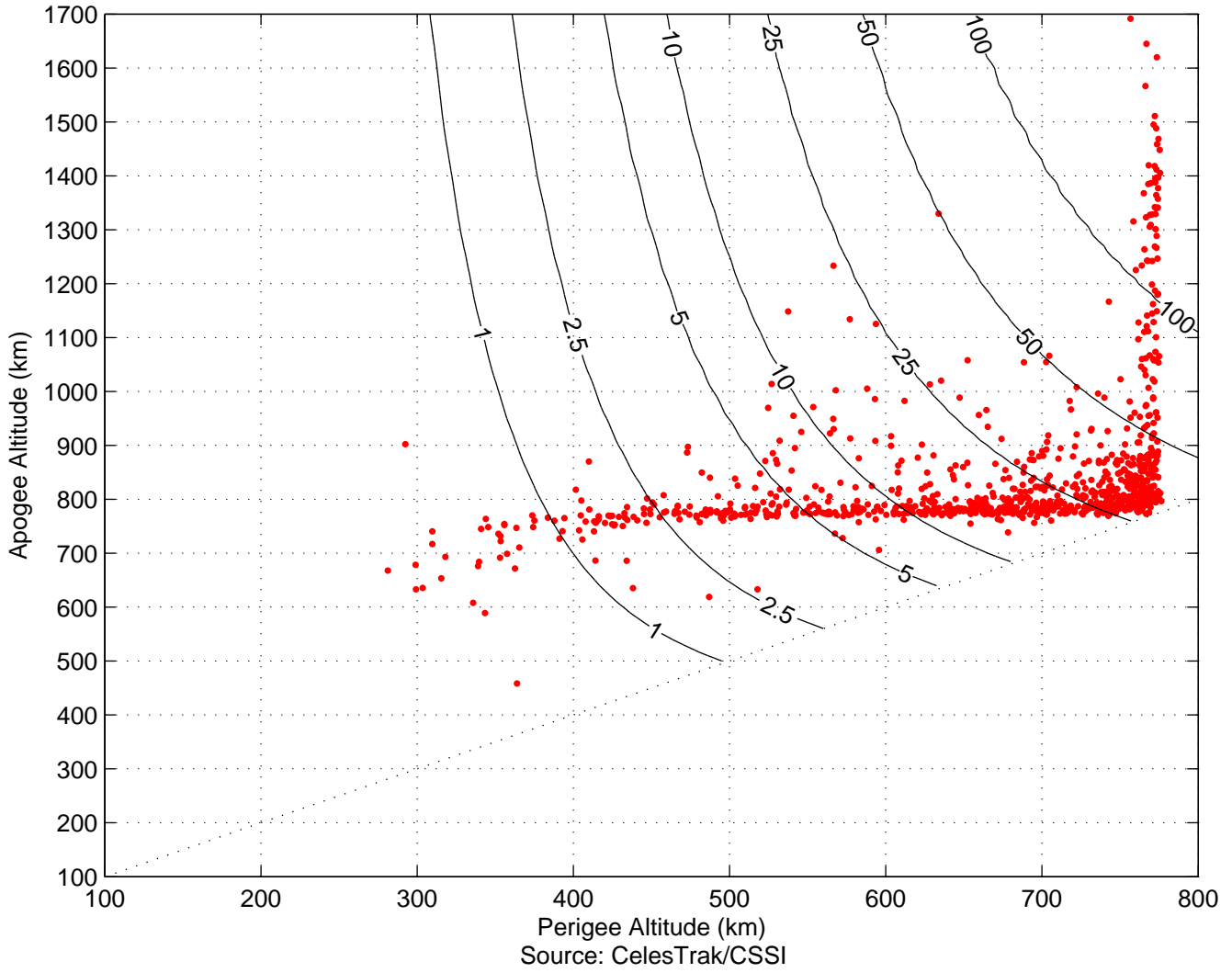
Apogee-Perigee Lifetime Plot of Cosmos 2251 Debris (961 pieces, 5-cm radius)
