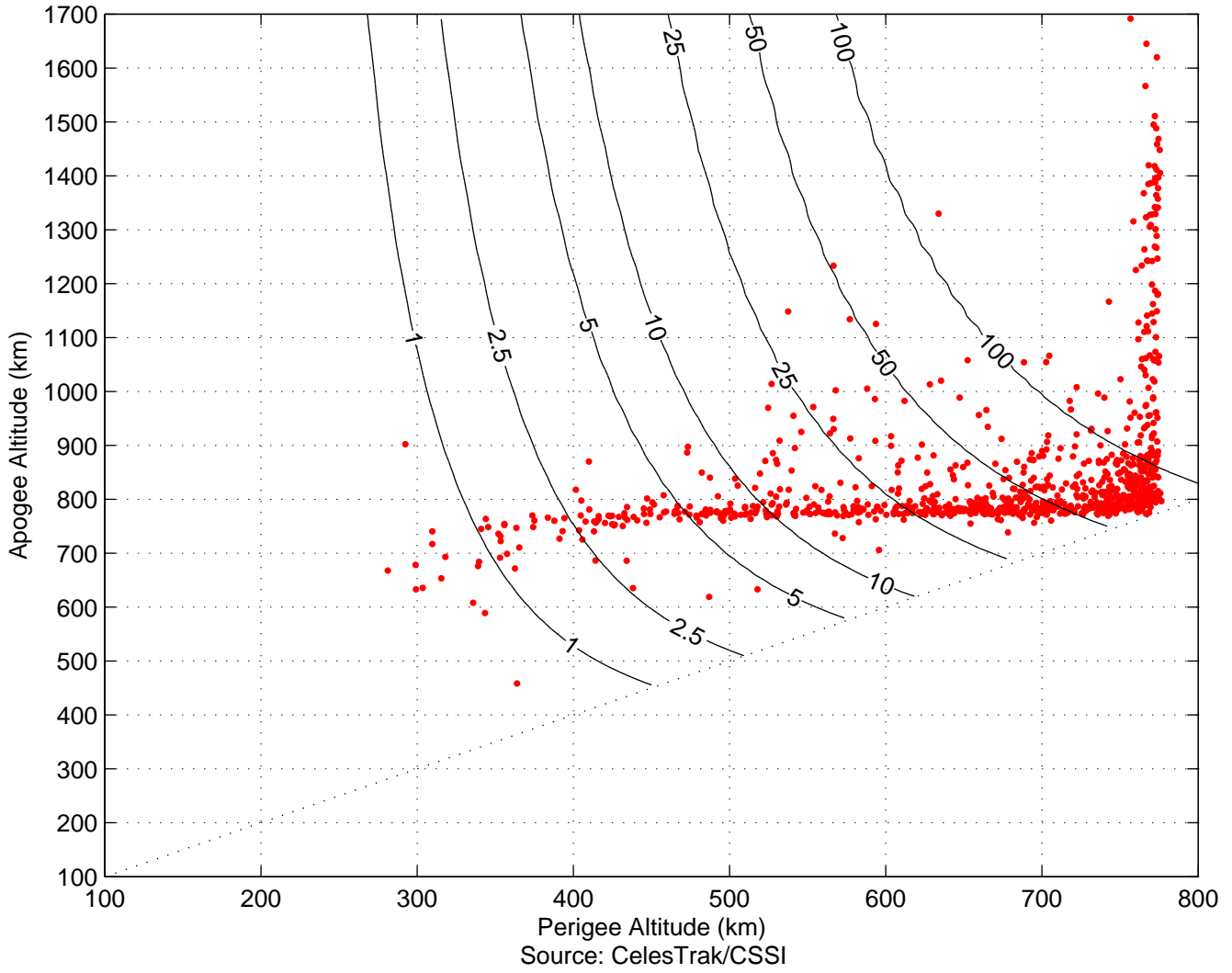
Apogee-Perigee Lifetime Plot of Cosmos 2251 Debris (961 pieces, average radius)
