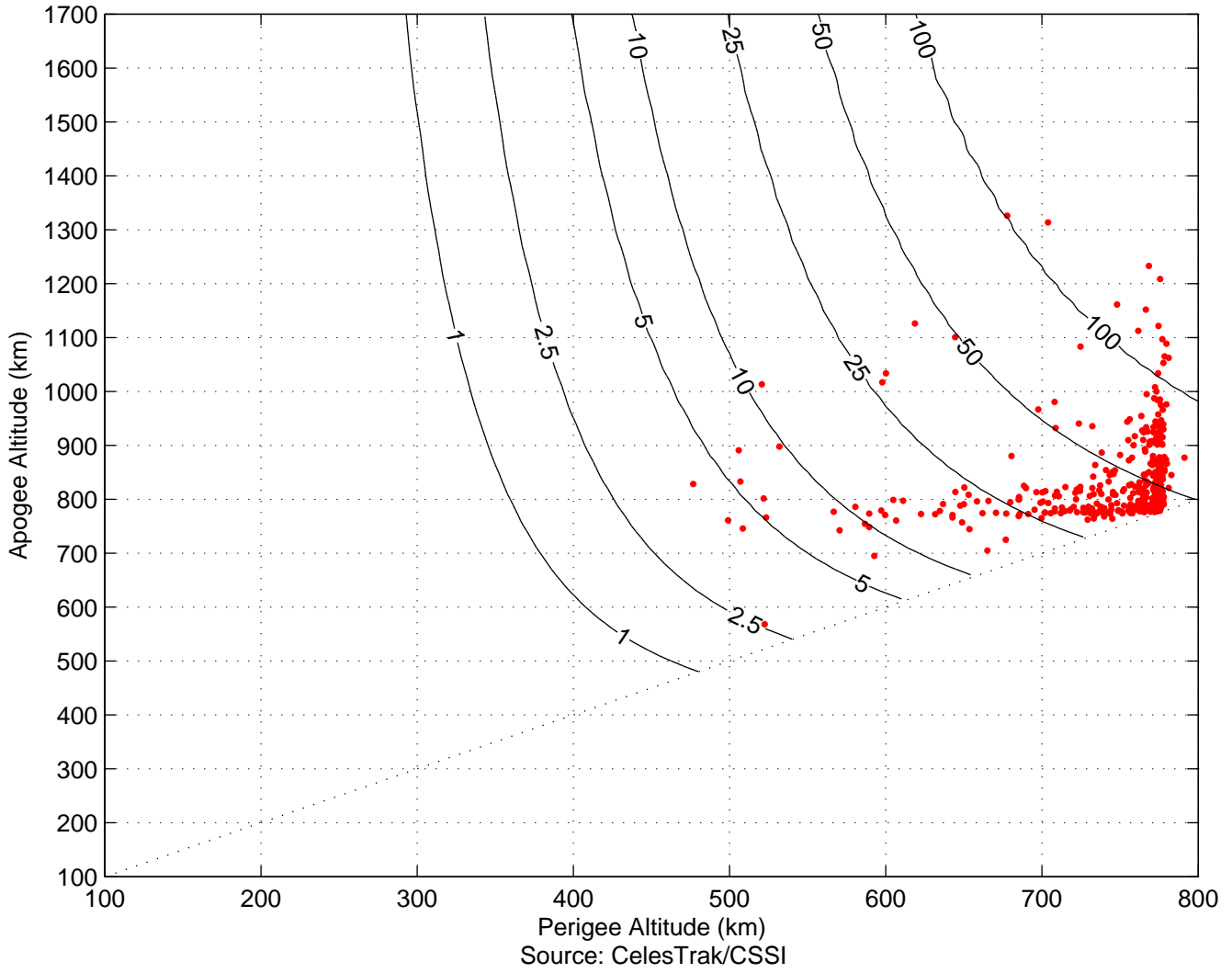
Apogee-Perigee Lifetime Plot of Iridium 33 Debris (398 pieces, 5-cm radius)
