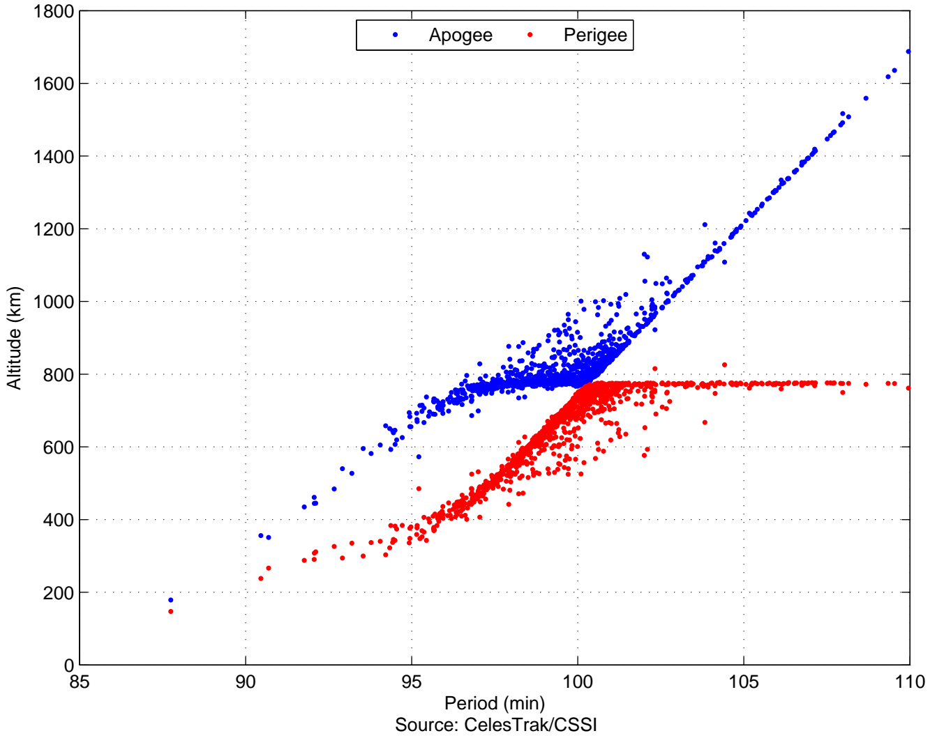
Gabbard Plot of Cosmos 2251 Debris (1208 pieces)
