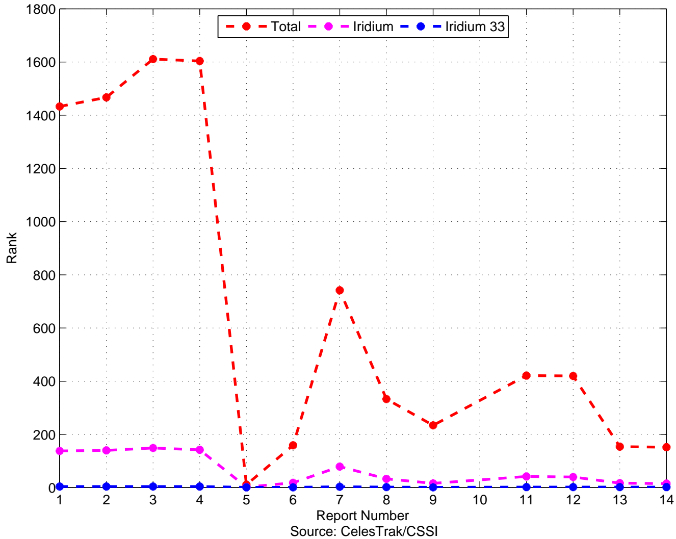
SOCRATES Rank
